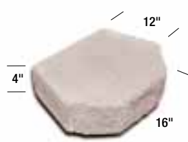
4" Beveled Cap 4 x 16 x 12 Weight: 50 lbs. Face Area: .44 sq. ft Units per Cube: 45
